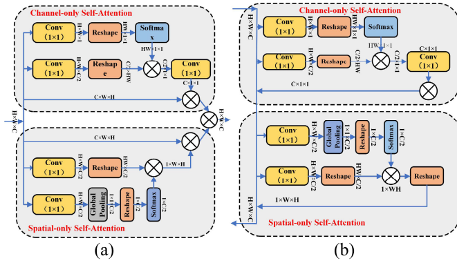
Fig. 3. PSA module. (a) Parallel structure of PSA. (b) Series structure of PSA.
