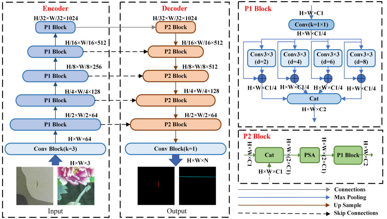
Fig. 2. Pipeline of PUNet and the individual module structures.
